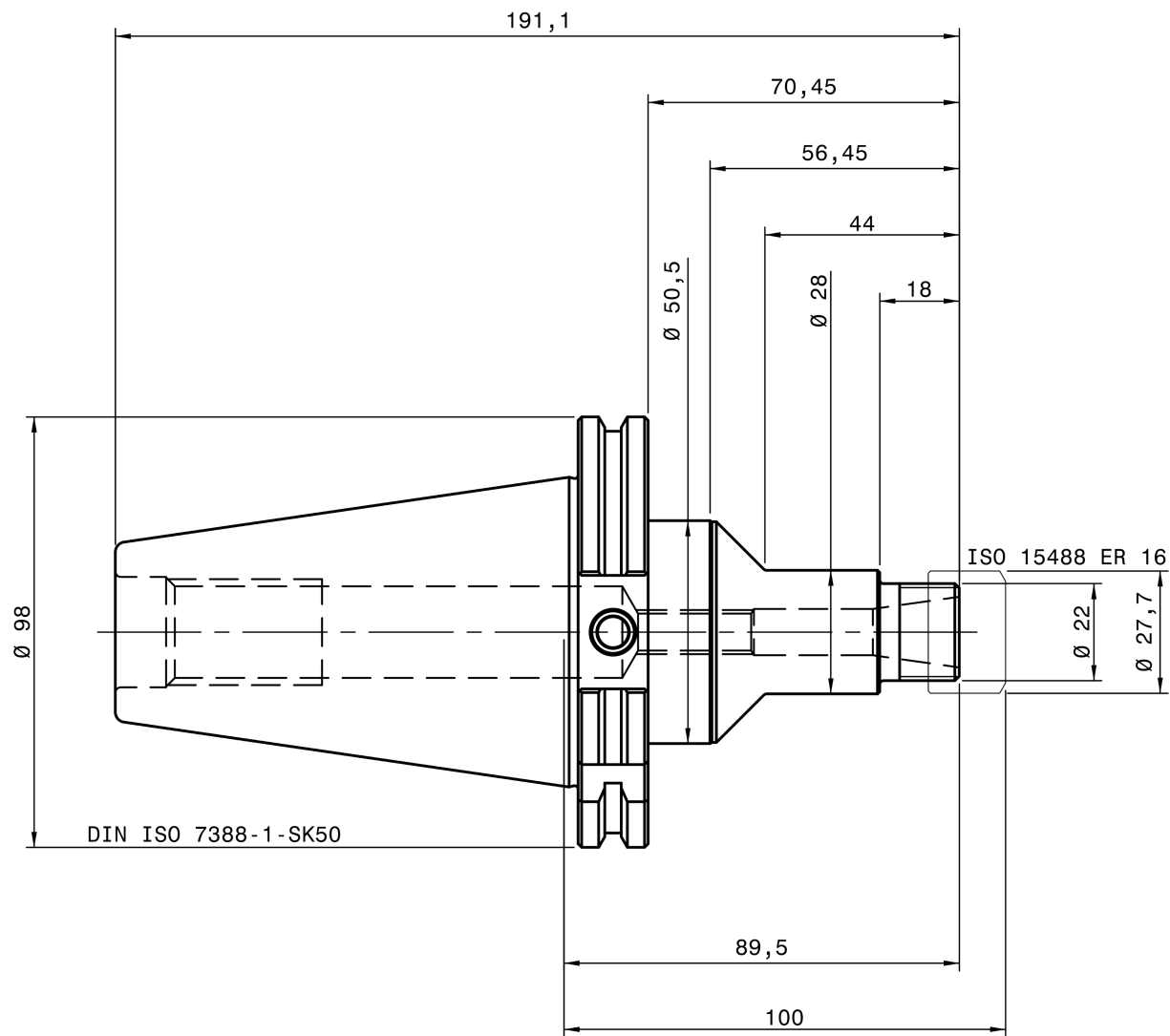
REGO-FIX B 4250.11653
